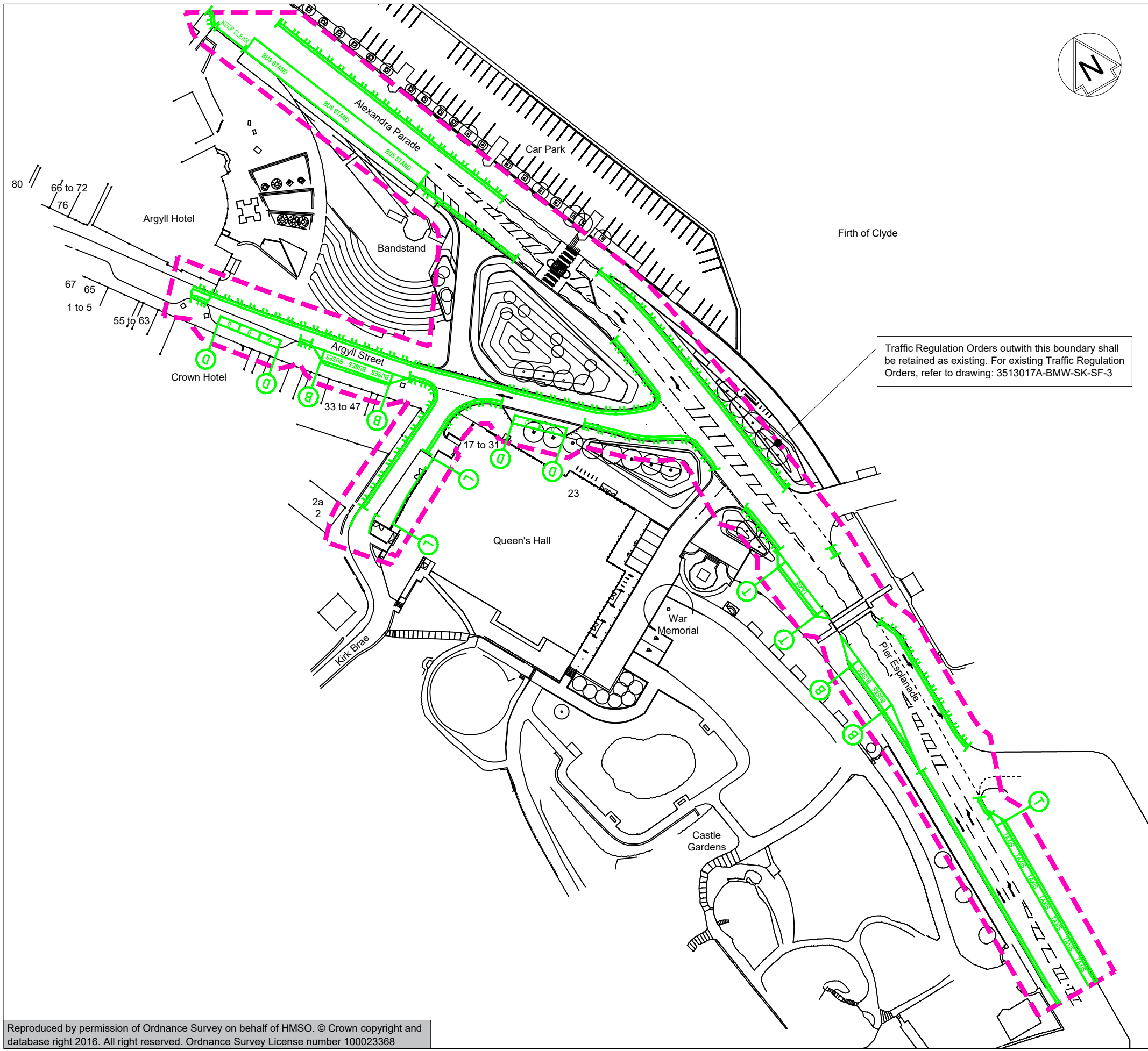
PLAN (Scale 1:1000)
