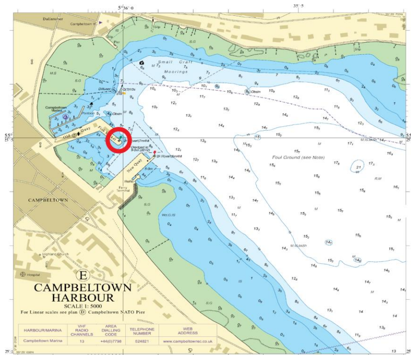
FIG: RED CIRCLE DENOTES POSITION OF LIGHTS
