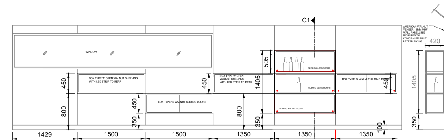
SECTION C1-C1
